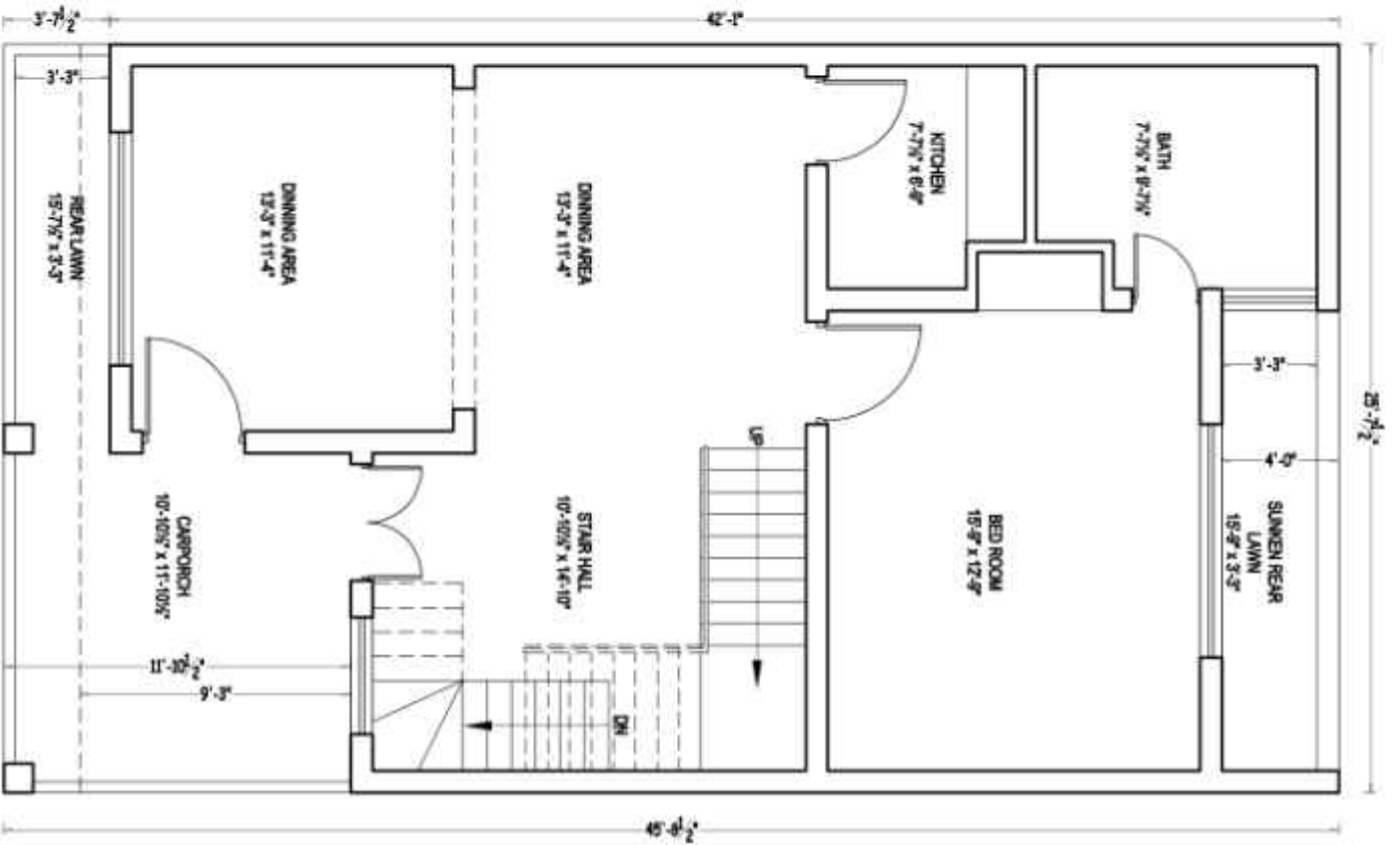
GROUND FLOOR PLAN COVERED AREA = 1038.0 SF
