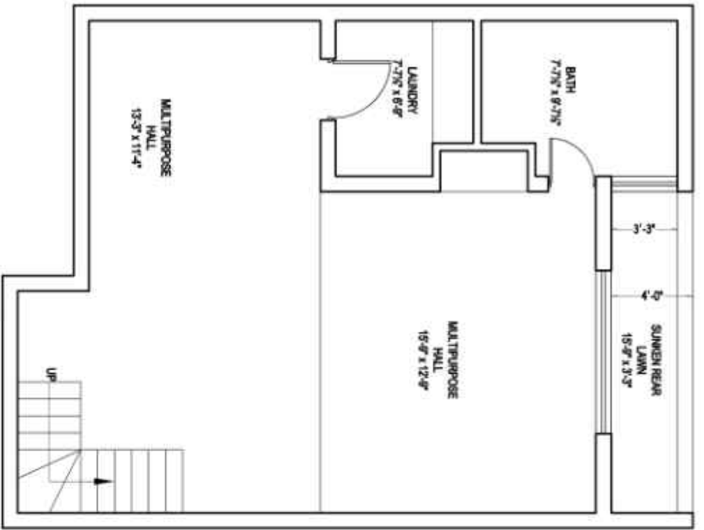
BASEMENT FLOOR PLAN COVERED AREA = 754.60 SF
